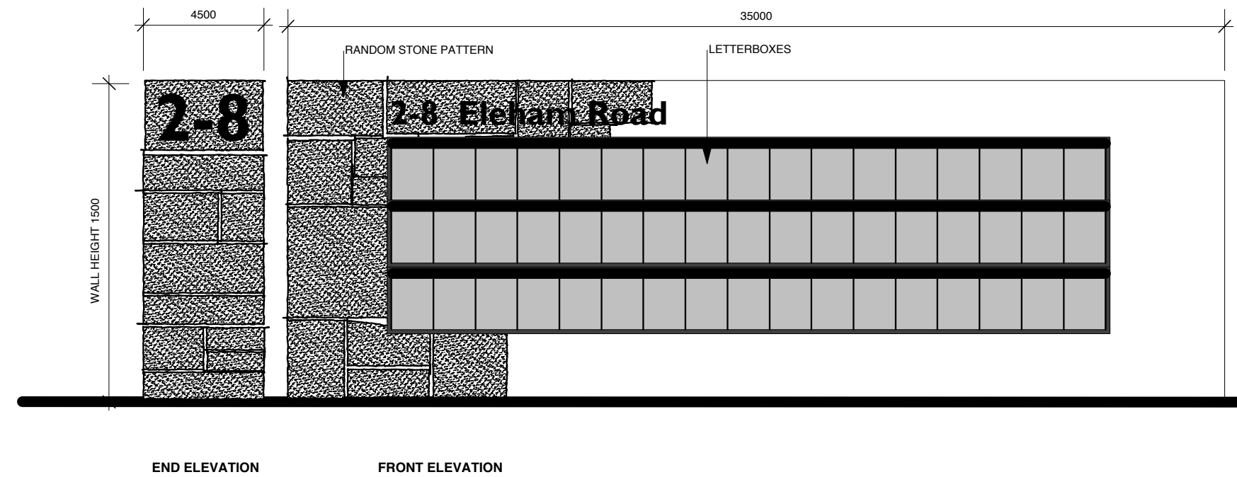
STONE ENTRY LETTERBOX WALL SCALE 1:20
