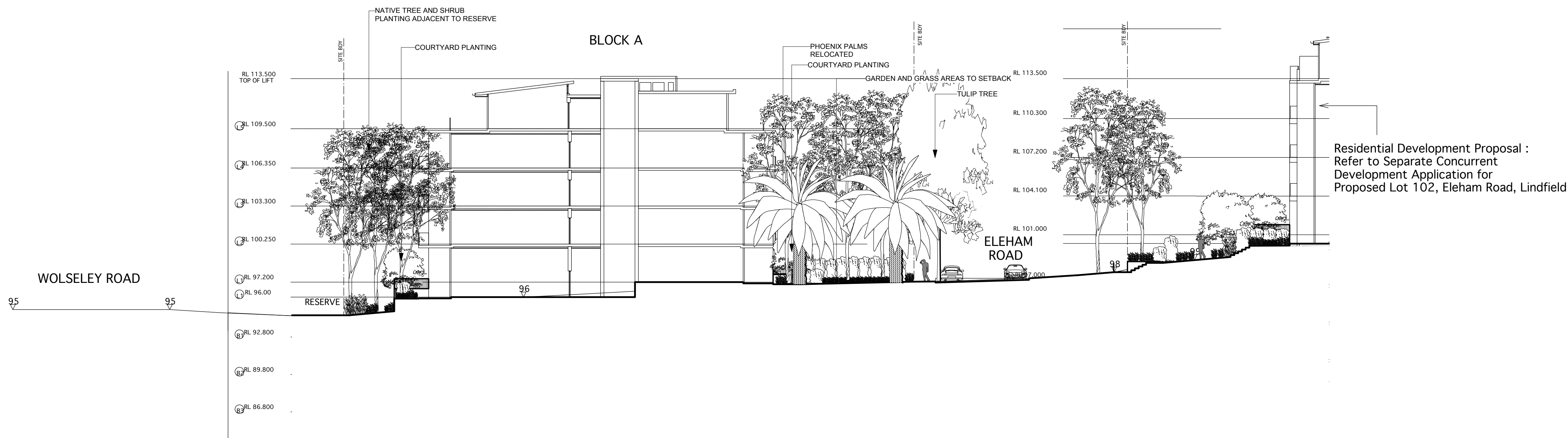
2 BLOCK A SECTION SCALE 1:200
